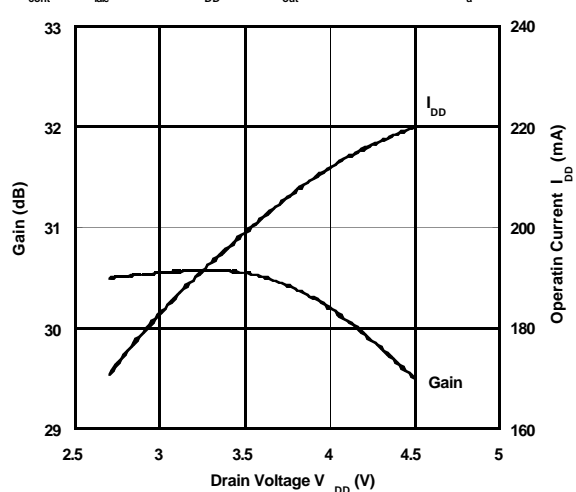
Gain, Operating Current vs. V_{DD}
