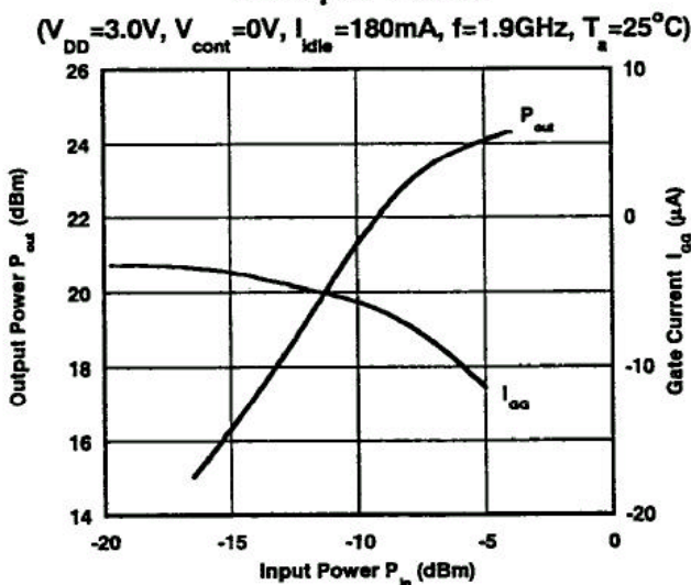
Output Power, Gate Current vs. Input Power
