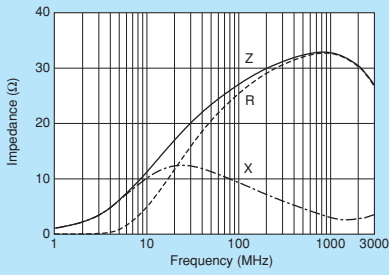
BLM18SG260TN1
