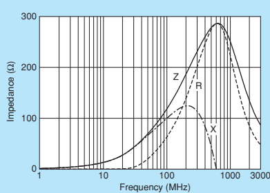
BLM18BD121SN1
