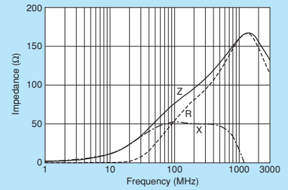
BLM03BD750SN1
