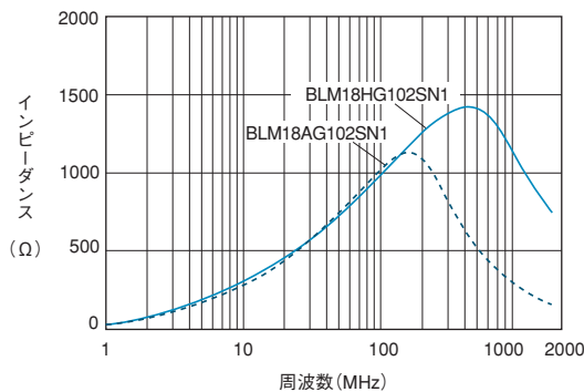
BLM18HG102SN1とBLM18AG102SN1 (従来品) の比較
