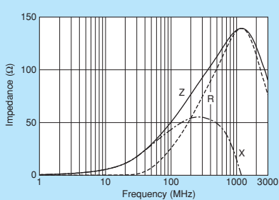
BLM18BD470SN1
