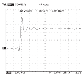
拡大 (10nsec/div, 2V/div)
