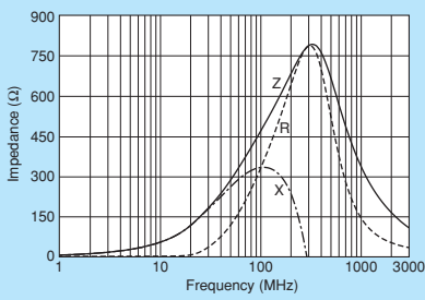
BLM15BX471SN1
