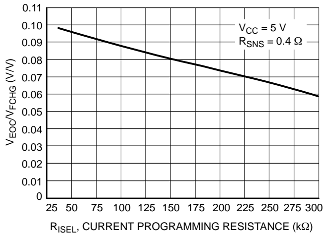
Figure 12. V EOC /V FCHG versus Current Programming Resistor
