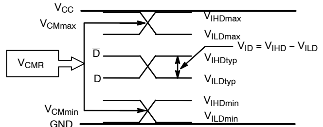
Figure 10. Differential Inputs Driven Differentially
