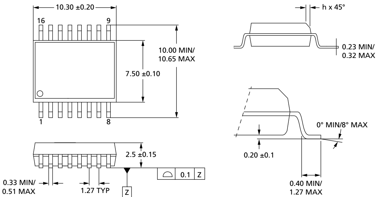
Figure 48: SOP2-16/300 mils
