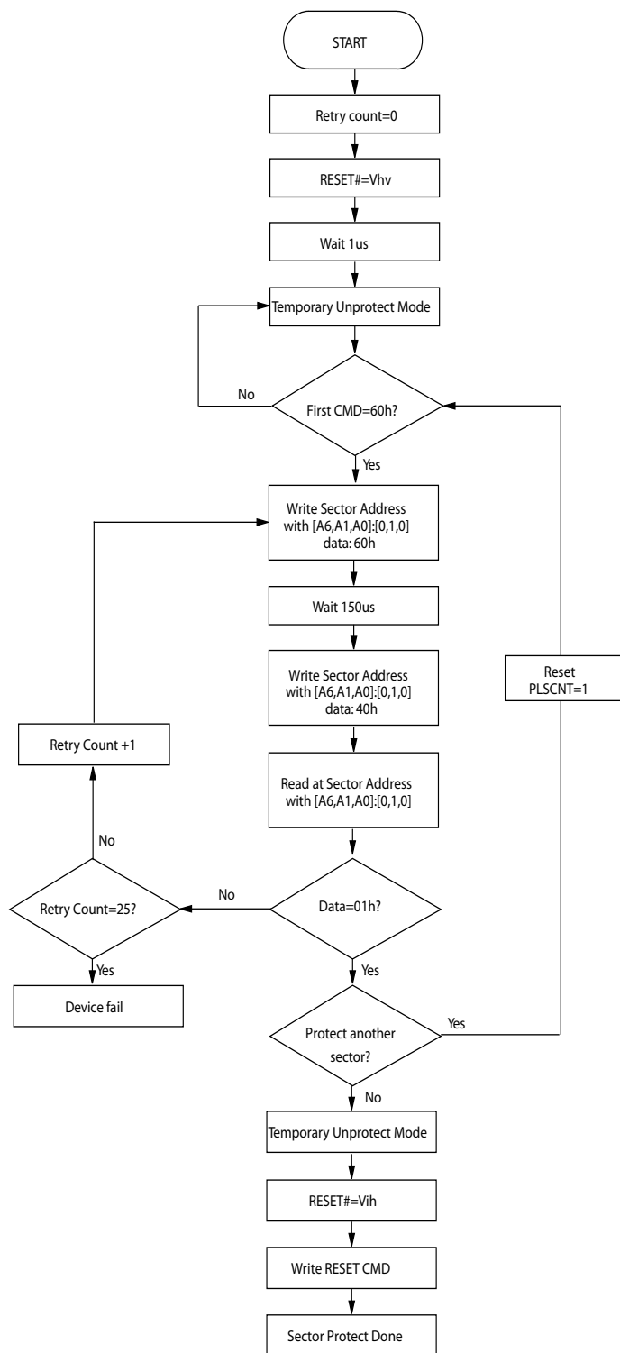
Figure 14. IN-SYSTEM SECTOR PROTECT WITH RESET# = Vhv
