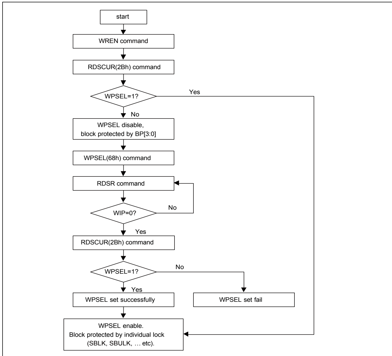
Figure 51. WPSEL Flow
