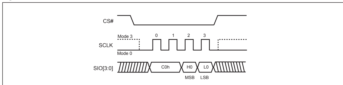
Figure 36. QPI Mode
