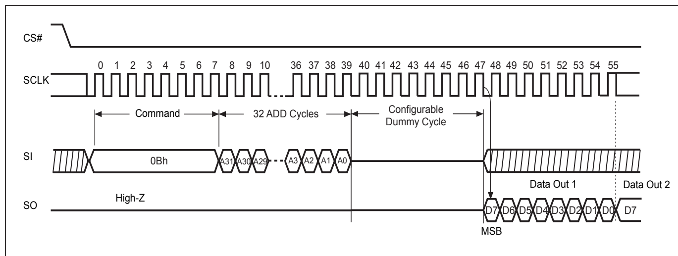
Figure 29. Read at Higher Speed (FAST_READ) Sequence (SPI Mode)
