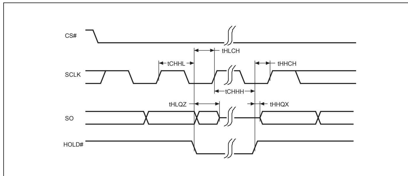
Figure 7. Hold Timing
