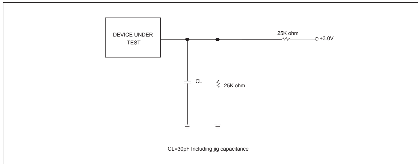
Figure 75. OUTPUT LOADING
