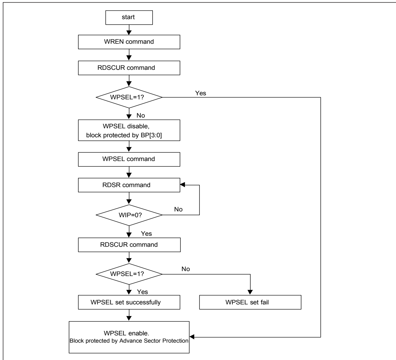
Figure 54. WPSEL Flow
