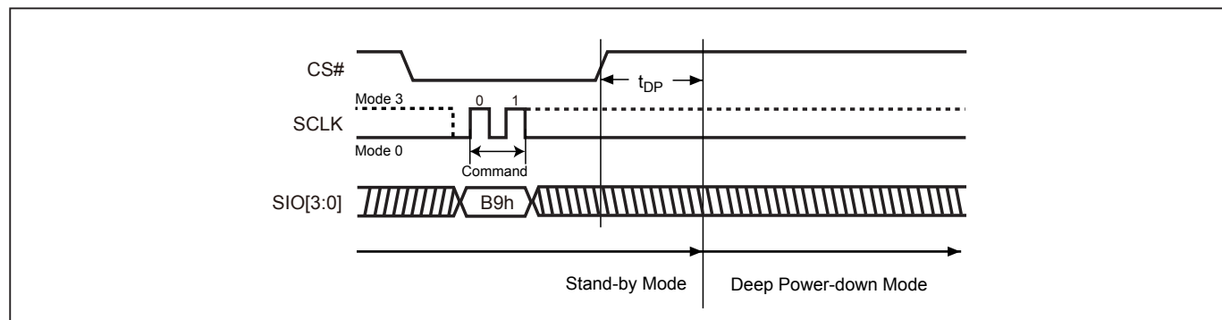
Figure 53. Deep Power-down (DP) Sequence (QPI Mode)
