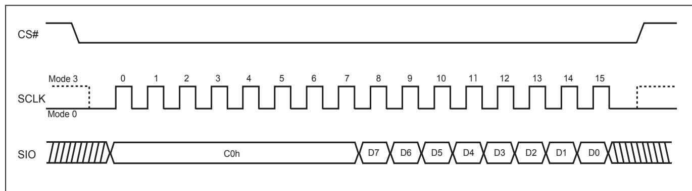
Figure 35. SPI Mode
