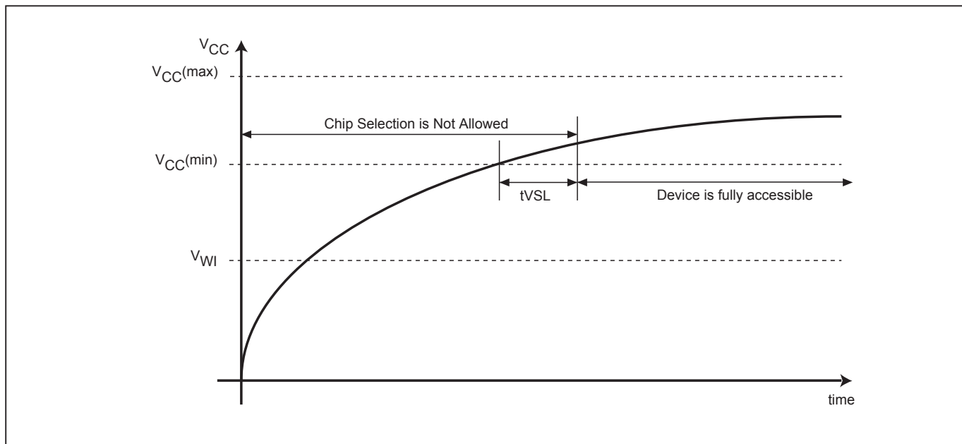
Figure 78. Power-up Timing
