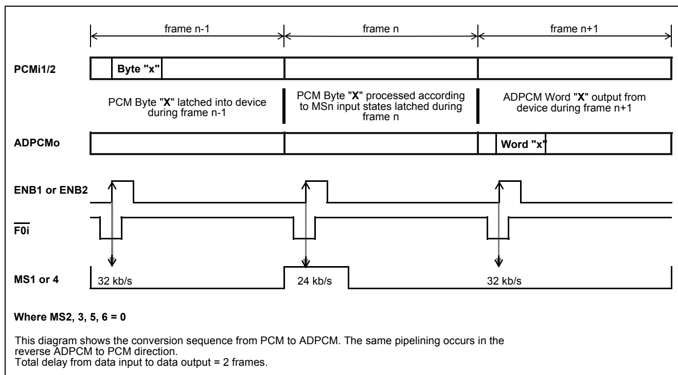
Figure 10 - Data Throughput
