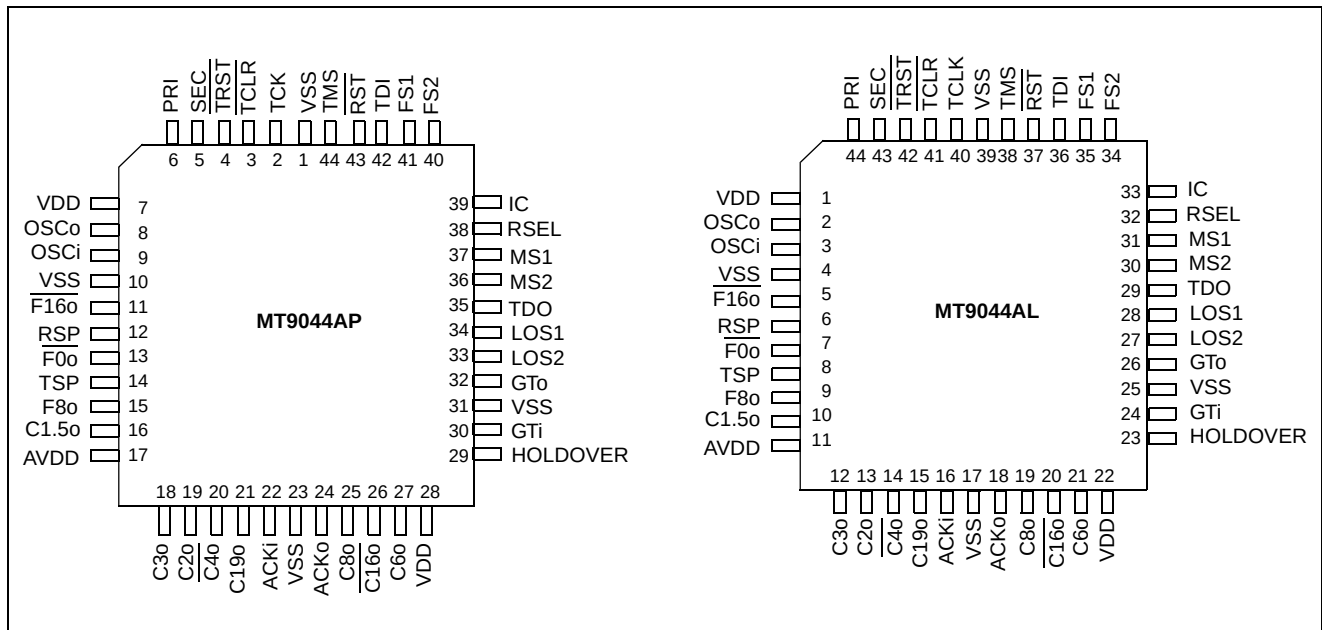
Figure 2 - Pin Connections
