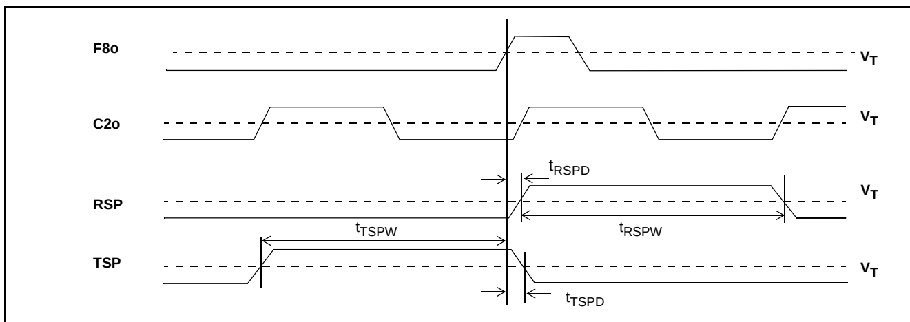
Figure 21 - Output Timing 2
