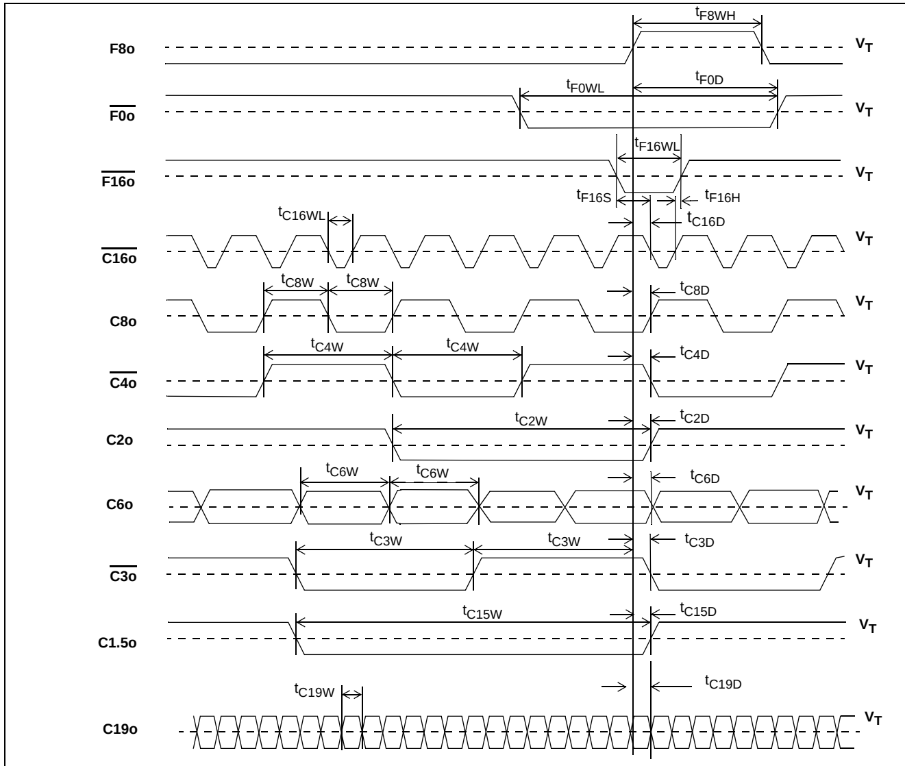
Figure 20 - Output Timing 1
