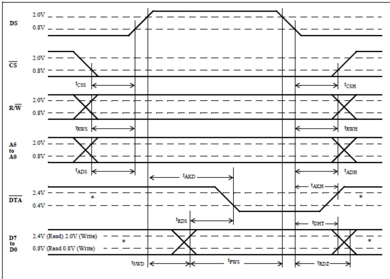
Figure 17 - Processor Bus
