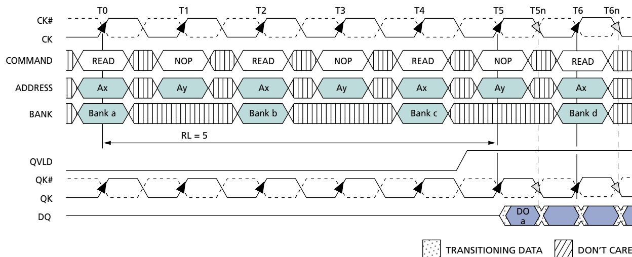
Figure 44: Consecutive READ Bursts with Multiplexed Addressing
