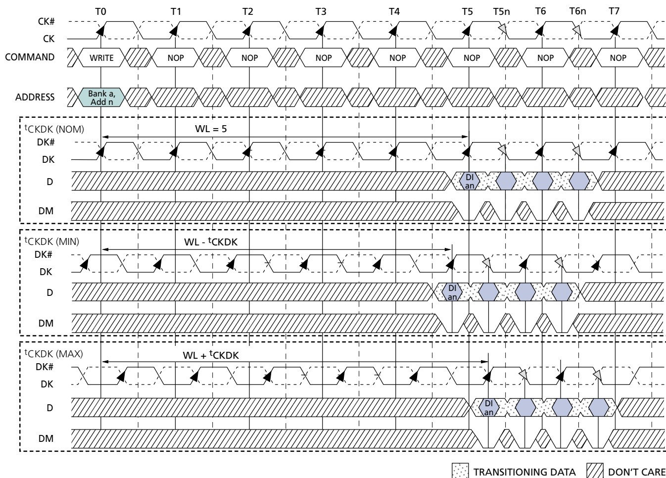
Figure 18: WRITE Burst
