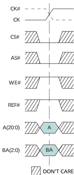
Figure 17: READ Command
