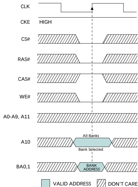
Figure 24: PRECHARGE Command
