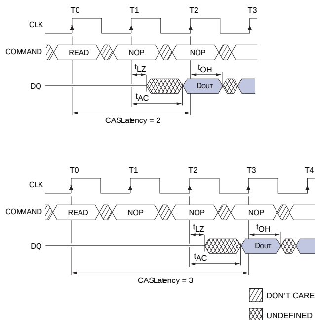
Figure 5: CAS Latency
