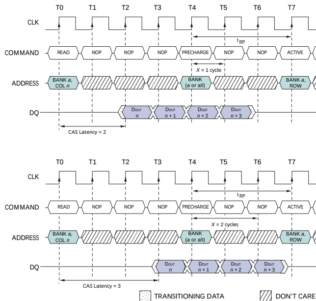
Figure 14: READ to PRECHARGE
