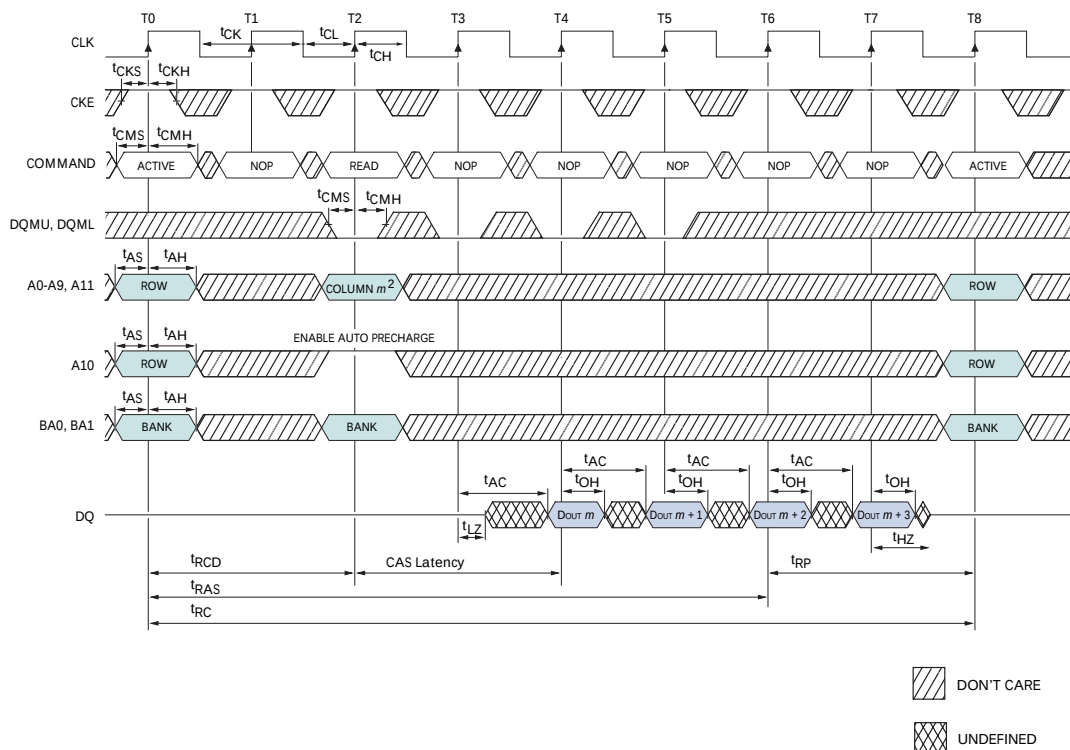
Figure 37: READ – With Auto Precharge 1
