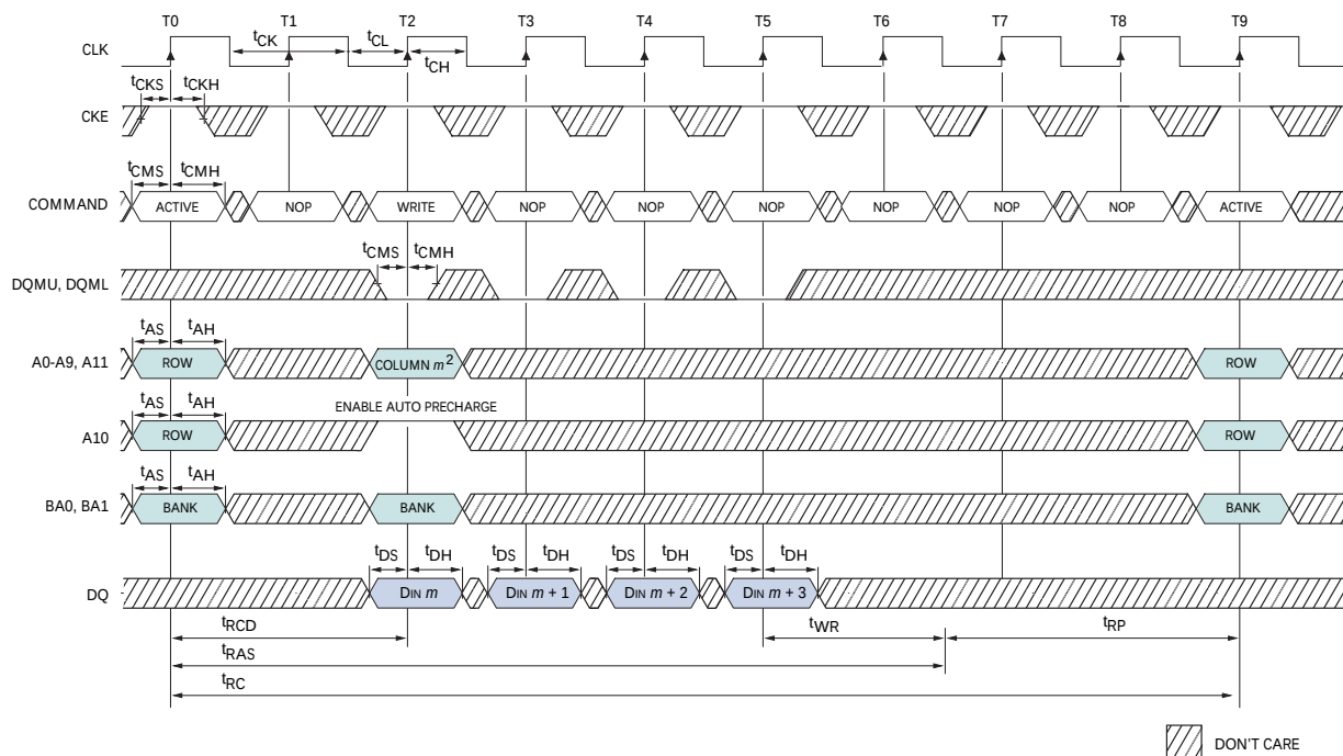
Figure 44: WRITE – With Auto Precharge 1
