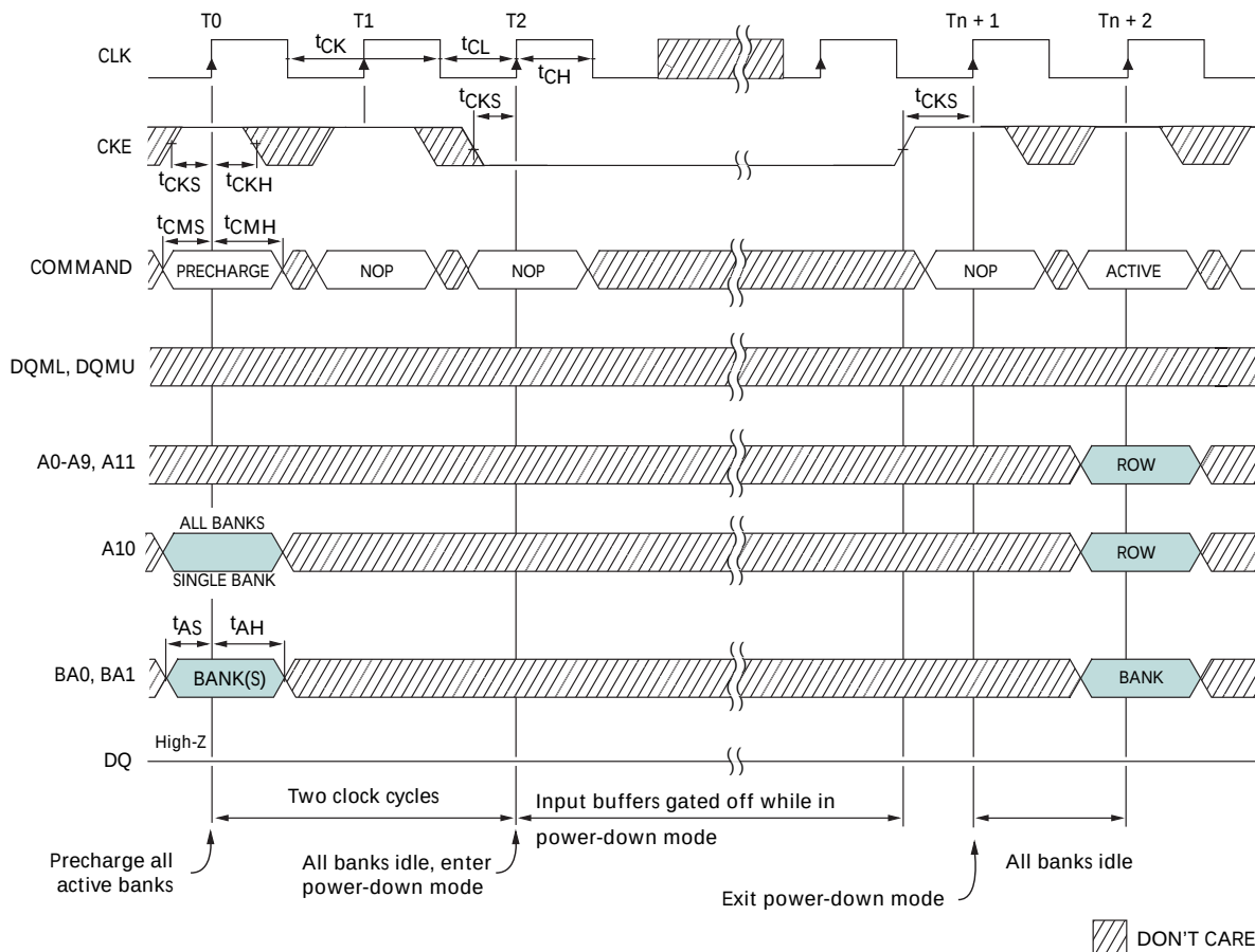
Figure 32: Power-Down Mode 1
