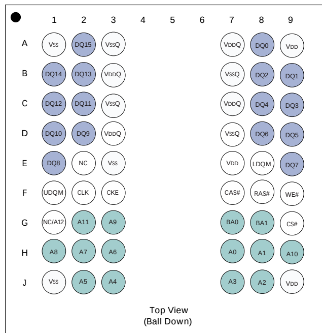
Figure 1: 54-Ball FBGA Pin Assignment (Top View)
