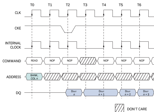
Figure 26: Clock Suspend During READ Burst
