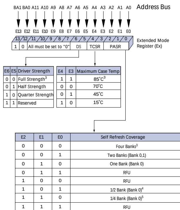
Figure 6: Extended Mode Register Table
