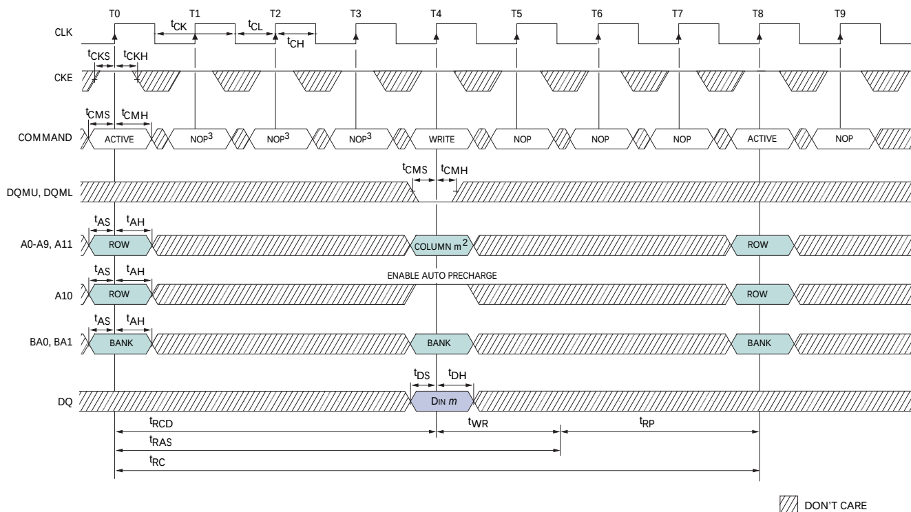
Figure 46: Single WRITE – With Auto Precharge 1
