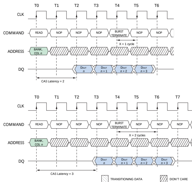
Figure 15: Terminating a READ Burst
