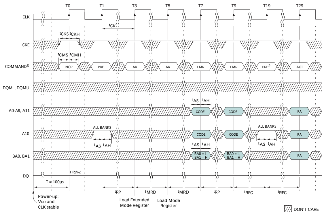
Figure 31: Initialize and Load Mode Register 1
