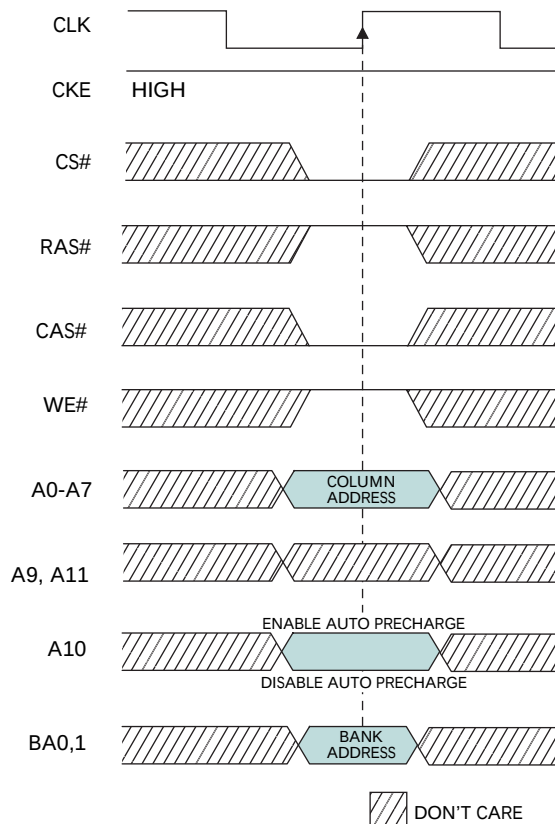
Figure 9: READ Command
