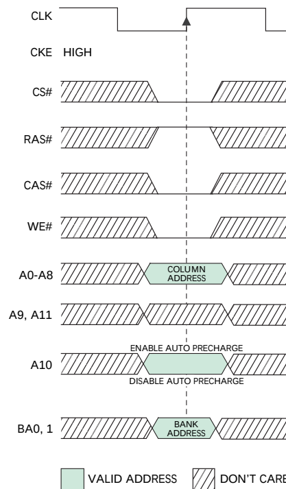
Figure 16: WRITE Command
