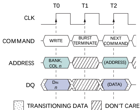
Figure 23: Terminating a WRITE Burst
