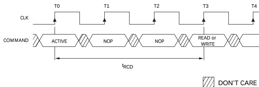
Figure 8: Meeting t_{RCD} (MIN) when 2 < t_{RCD} \text{ (MIN)} / t_{CK} \leq 3
