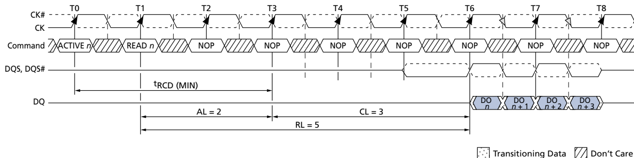
Figure 37: READ Latency
