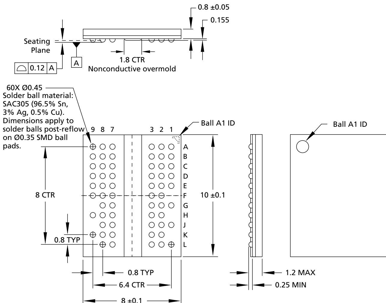
Figure 9: 60-Ball FBGA (8mm x 10mm) – x4, x8
