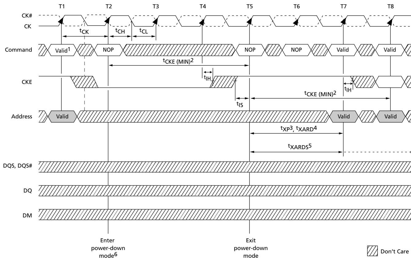
Figure 70: Power-Down
