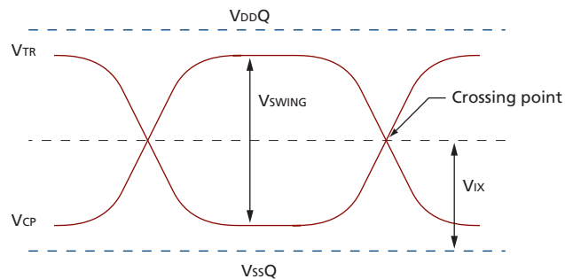
Figure 37: AC Input Test Signal Waveform (Differential)
