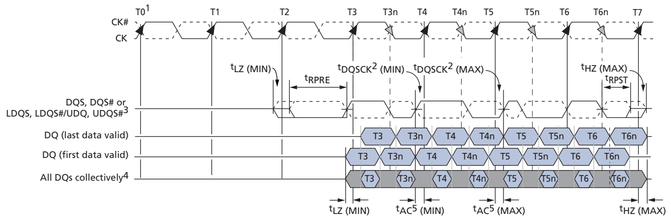
Figure 59: Data Output Timing – t_{AC} and t_{DQSCK}
