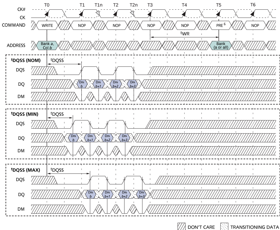
Figure 25: WRITE-to-PRECHARGE – Uninterrupting
