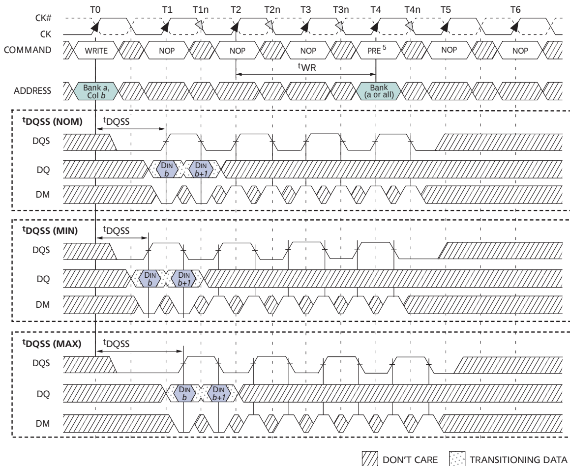
Figure 26: WRITE-to-PRECHARGE – Interrupting
