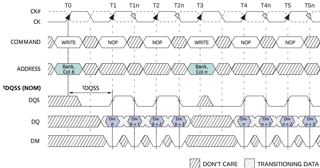
Figure 20: Nonconsecutive WRITE-to-WRITE
