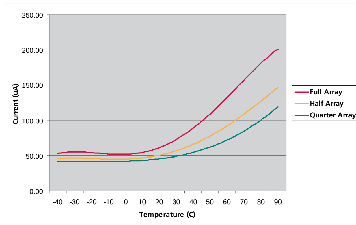
Figure 30: Typical Self-Refresh Current vs. Temperature
