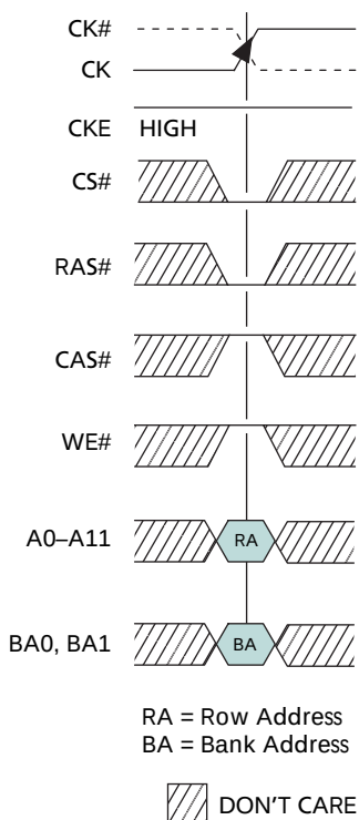
Figure 7: Activating a Specific Row in a Specific Bank
