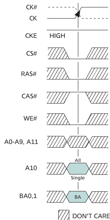
Figure 28: PRECHARGE Command
