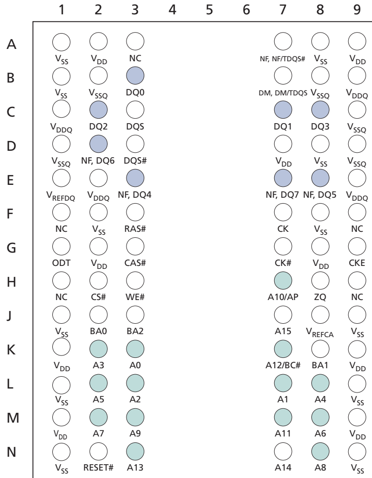
Figure 6: 78-Ball FBGA – x4, x8 (Top View)
