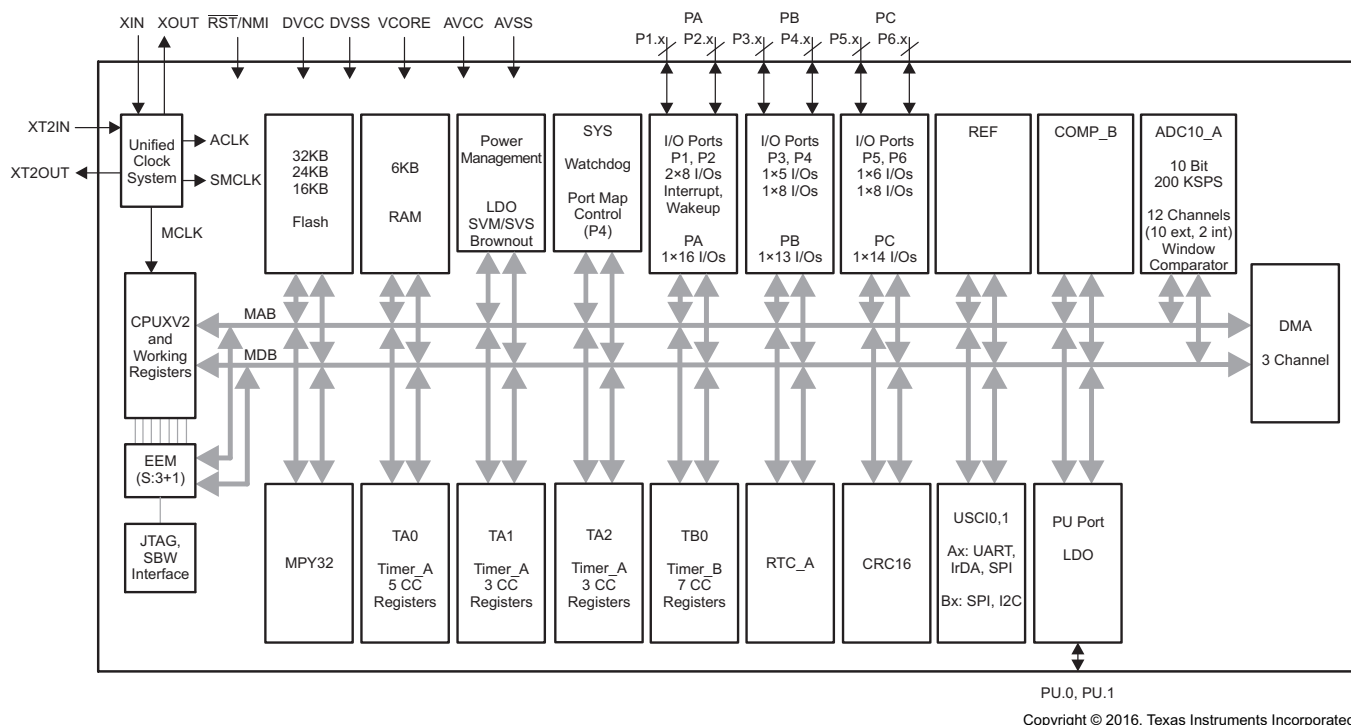
Figure 1-1. Functional Block Diagram – RGC, ZXH, or ZQE Package – MSP430F5310, MSP430F5309, MSP430F5308
