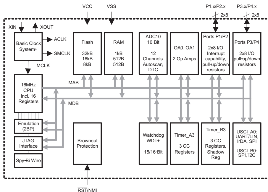
MSP430F22x4 Functional Block Diagram
