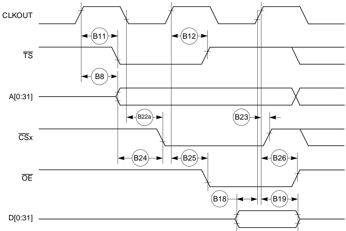
Figure 13. External Bus Read Timing (GPCM Controlled—TRLX = 0, ACS = 10)
