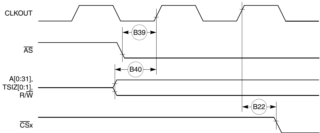
Figure 21. Asynchronous External Master Memory Access Timing (GPCM Controlled—ACS = 00)
