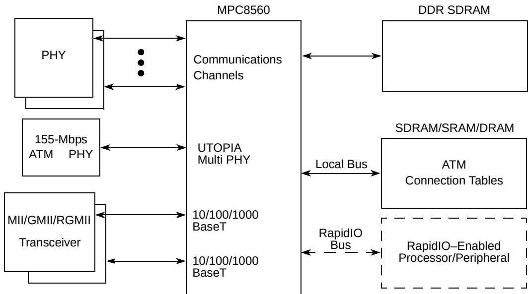
Figure 5. Basic System Configuration
