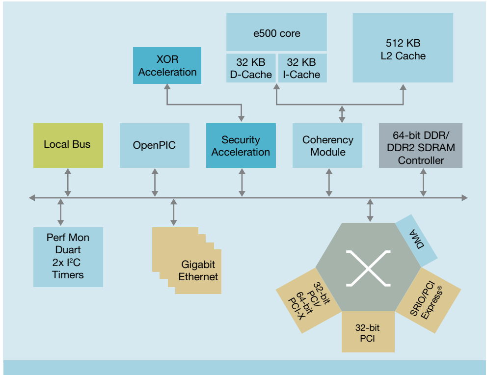
MPC8548/E Block Diagram
