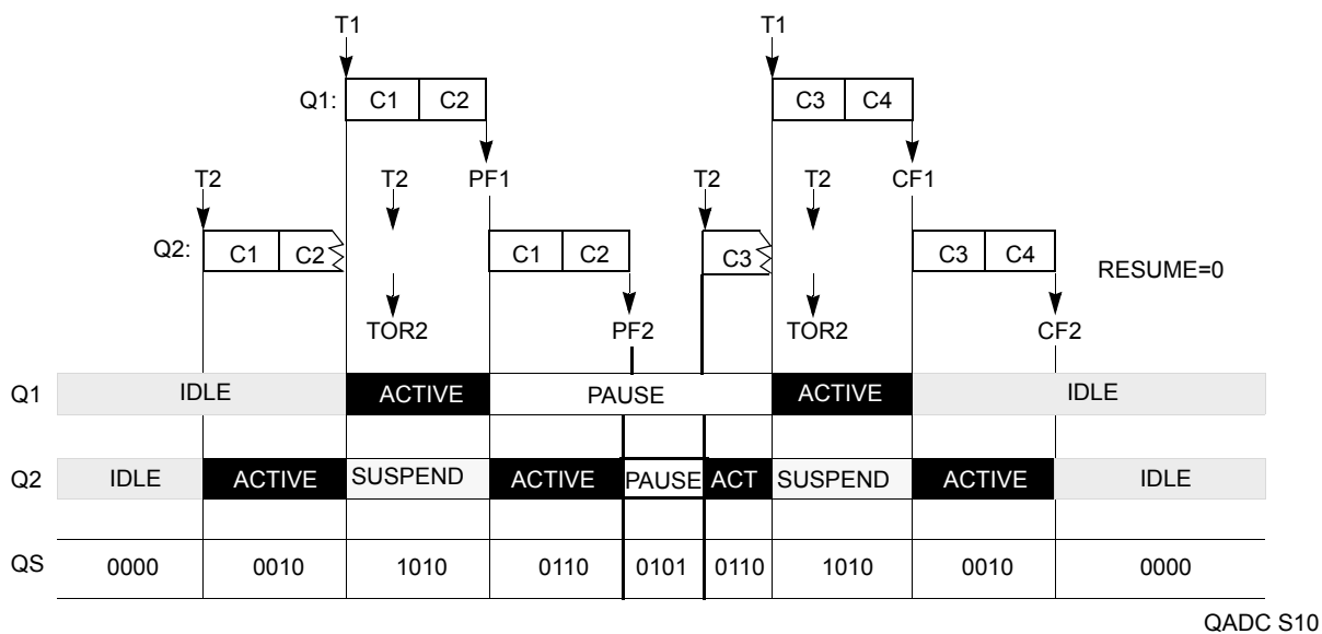
Figure 14-34. CCW Priority Situation 10
