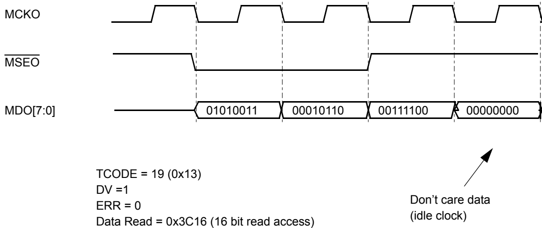
Figure 24-68. Upload/Download Information Message
