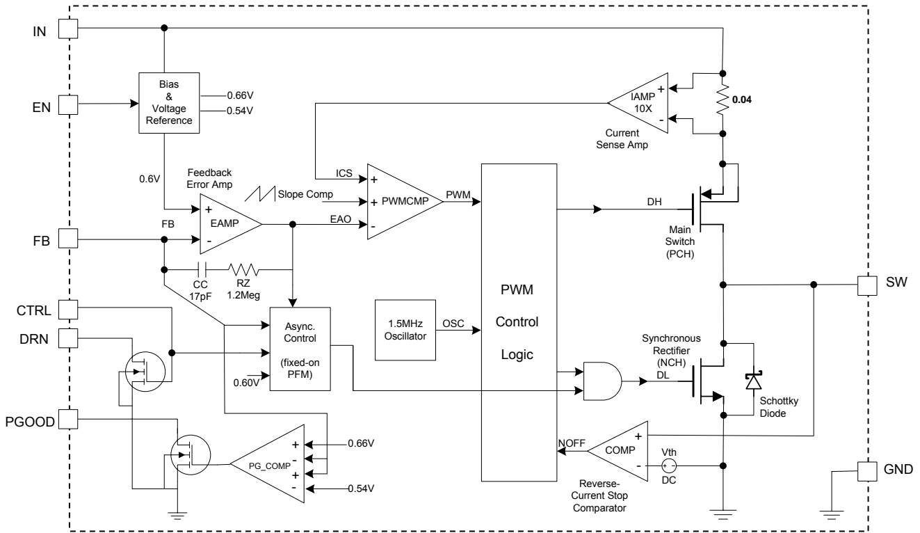
Figure 1-Functional Block Diagram
