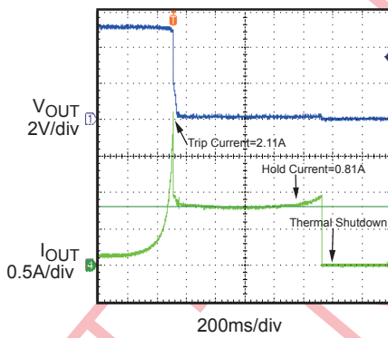
Current Limit R_{LIMIT} = 60\Omega
