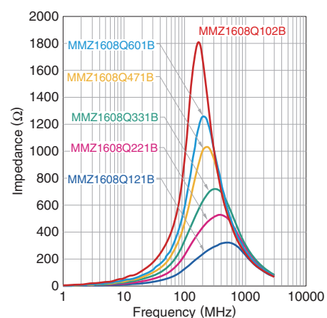
MMZ1608Q series
