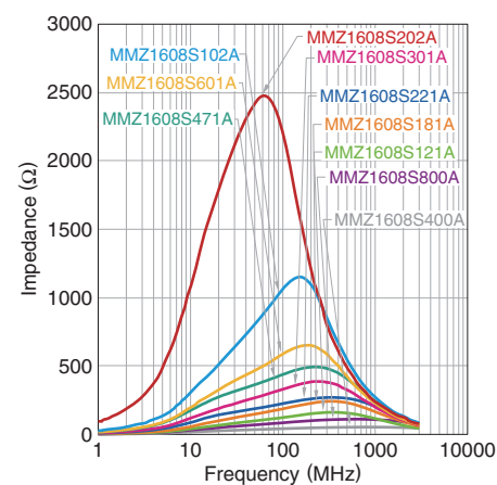
MMZ1608S series
