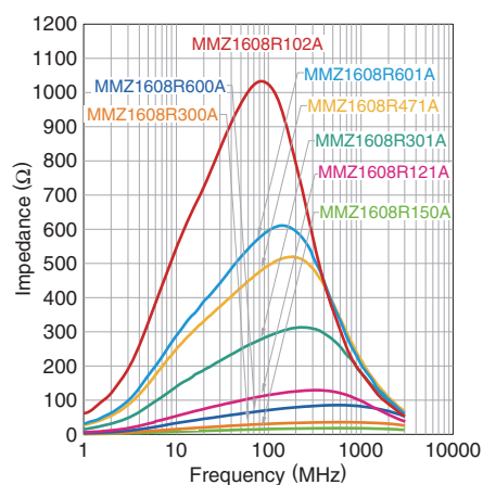
MMZ1608R series
