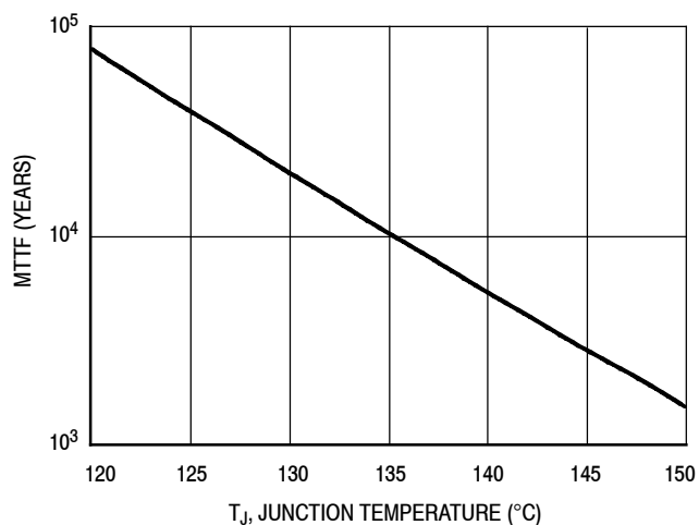
Figure 11. MTTF versus Junction Temperature NOTE: The MTTF is calculated with V_{CC} = 5 \text{ Vdc} , I_{CC} = 41 \text{ mA}
