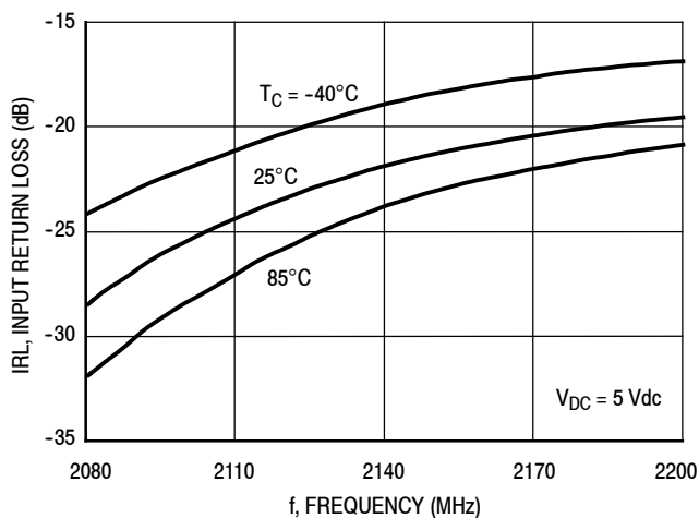
Figure 28. Input Return Loss (S11) versus Frequency
