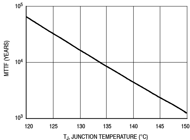
Figure 11. MTTF versus Junction Temperature NOTE: The MTTF is calculated with V_{CC} = 5.6 \text{ Vdc} , I_{CC} = 58 \text{ mA}
