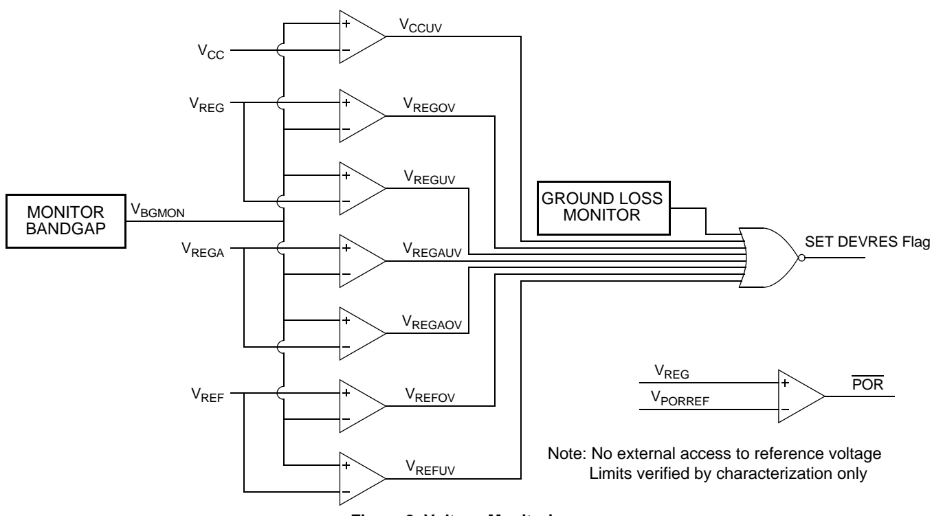
Figure 9. Voltage Monitoring
