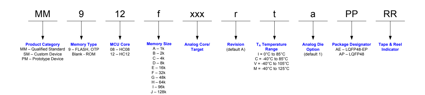
Figure 2. Part Number Scheme
