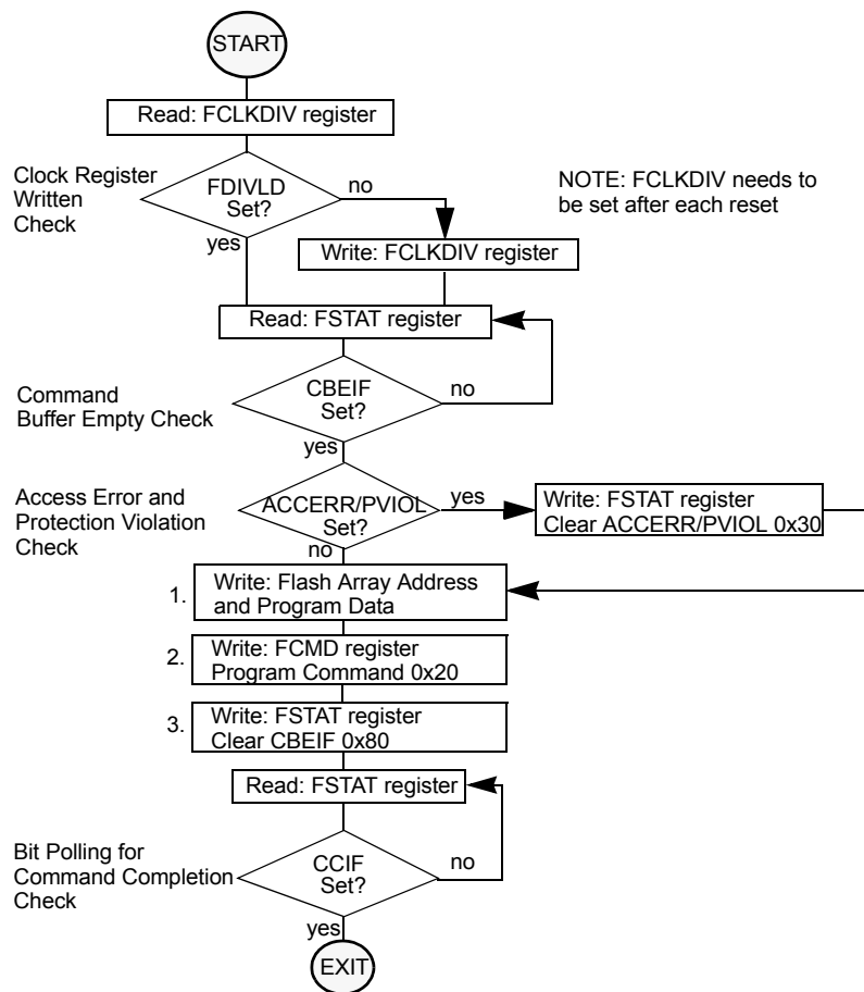
Figure 85. Example Program Command Flow
