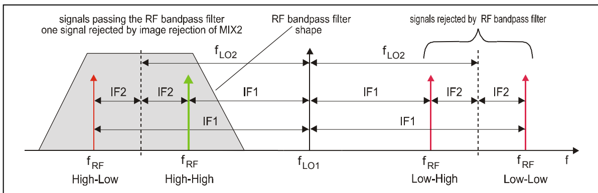
Fig. 3: The four receiving frequencies in a double conversion superhetro receiver
