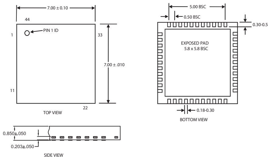
44-PIN (7 x 7 x 1mm) LPCC
