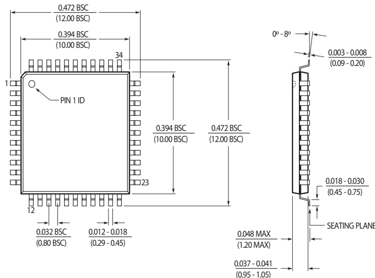
Package: H44-10 44-Pin (10 x 10 x 1mm) TQFP
