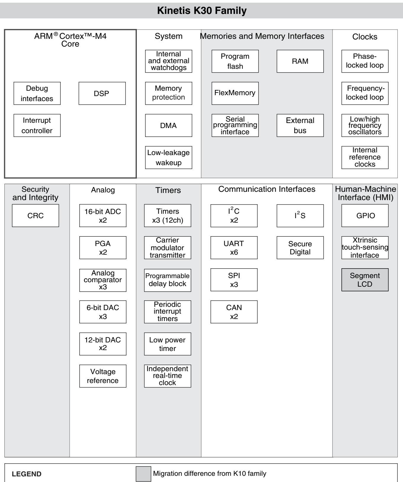
Figure 2. K30 Block Diagram
