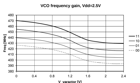
Figure 7. RF Frequency vs. Varactor Voltage and VCO Frequency bit ( V_{DD} = 2.5V )
