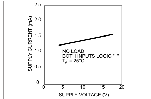
FIGURE 2-10: Quiescent Power Supply Current vs. Supply Voltage.
