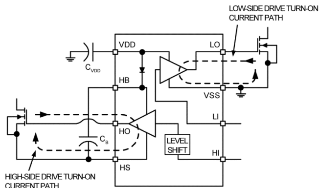
Figure 9. Turn-Off Current Paths
