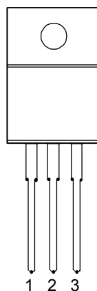
MIC29510BT/WT
