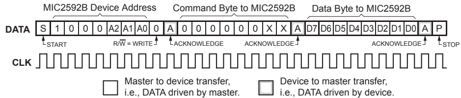
Figure 10. WRITE_BYTE Protocol
