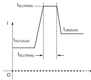
Figure 5. VAUX Current Limit Response Timing
