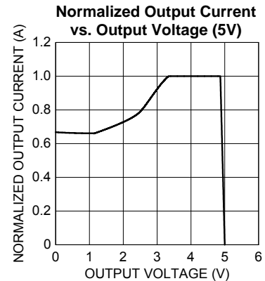
Figure 6. Normalized Output Current vs. Output Voltage
