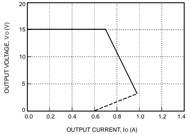
Figure 15. ME005C Typical Output Characteristics with V_i = 48 V and T_A = 25 °C
