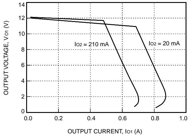
Figure 16. ME005BK Typical Output Characteristics ( V_{o1} vs. I_{o1} ) with V_i = 48 V and T_A = 25 °C
