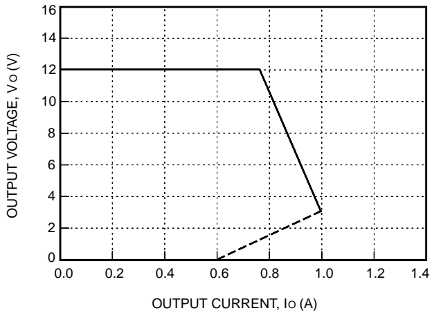
Figure 14. ME005B Typical Output Characteristics with V_i = 48 V and T_A = 25 °C
