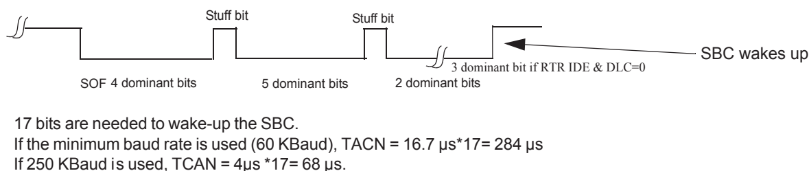
Figure 43. CAN Frame with 11 Bits of Identifier Field at 0
