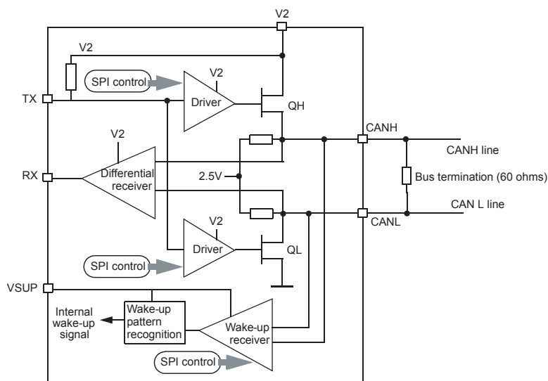
Figure 34. 33989 CAN Interface
