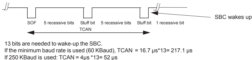
Figure 42. CAN Frame with 11 Bits of Identifier Field at 1
