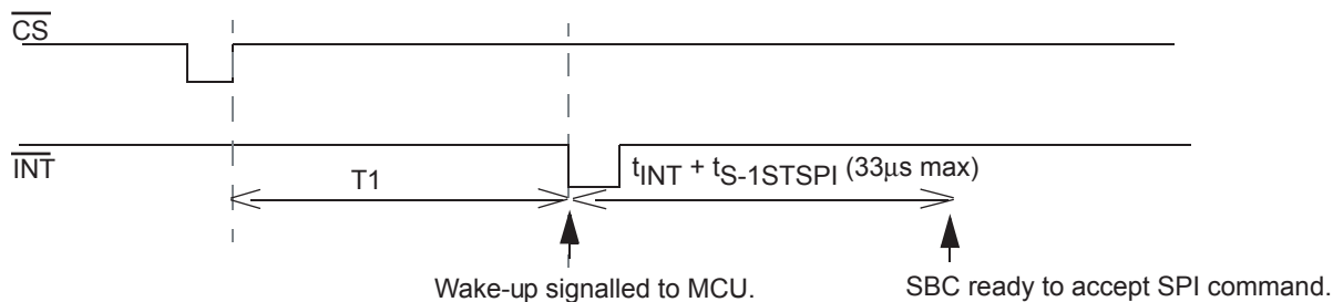
Figure 31. \overline{\text{CS}} Wake-up
