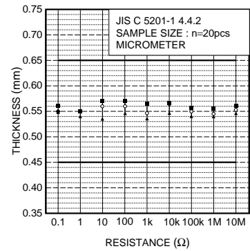
Fig.4 Dimensions (thickness)
